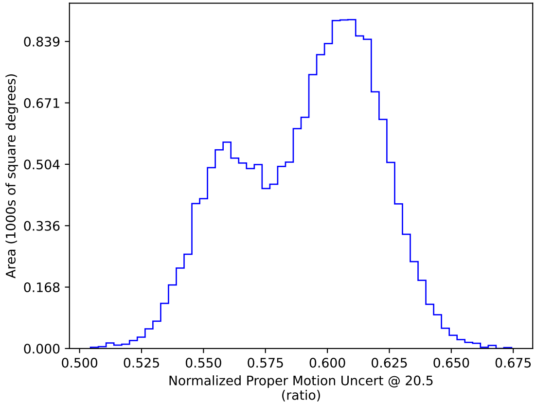
too_elab_heavy_r64_d2_gz_v3.4_10yrs WFD: Normalized Proper Motion Uncert @ 20.5
