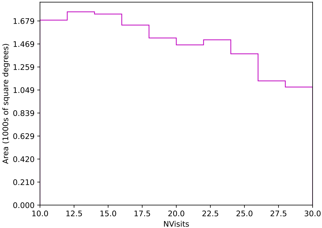
too_elab_heavy_r64_d2_gz_v3.4_10yrs Yr 3-4 z band: NVisits
