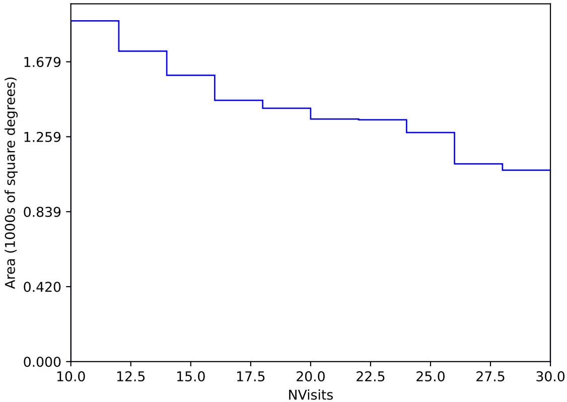
too_elab_heavy_r64_d2_gz_v3.4_10yrs Yr 3-4 y band: NVisits
