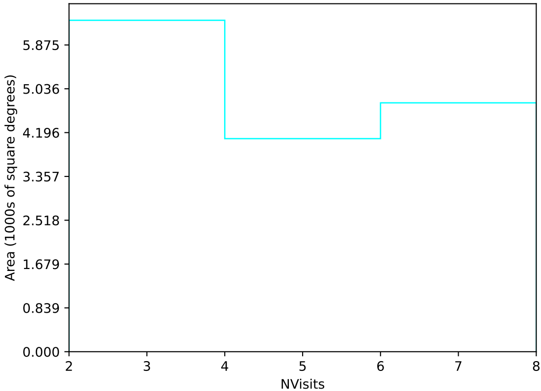
too_elab_heavy_r64_d2_gz_v3.4_10yrs Yr 3-4 u band: NVisits
