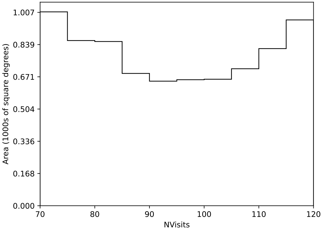
too_elab_heavy_r64_d2_gz_v3.4_10yrs Yr 3-4 all bands: NVisits
