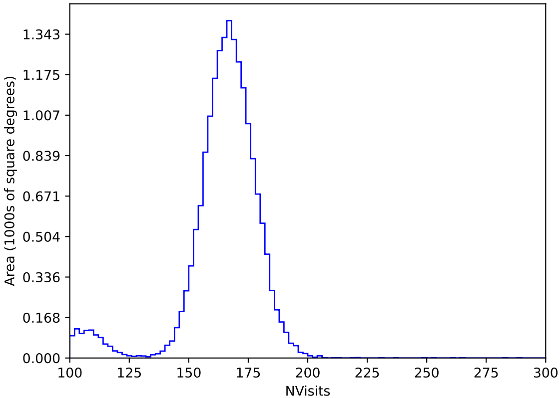
too_elab_heavy_r64_d2_gz_v3.4_10yrs WFD y band: NVisits
