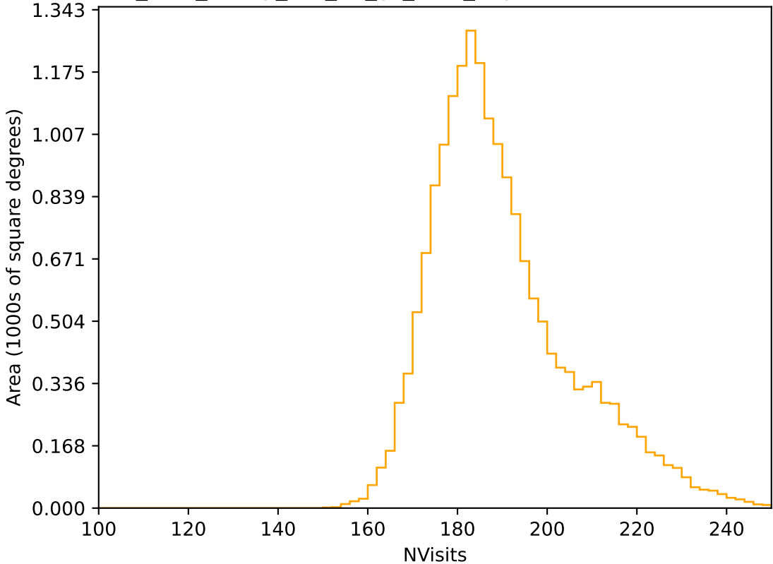
too_elab_heavy_r64_d2_gz_v3.4_10yrs WFD r band: NVisits
