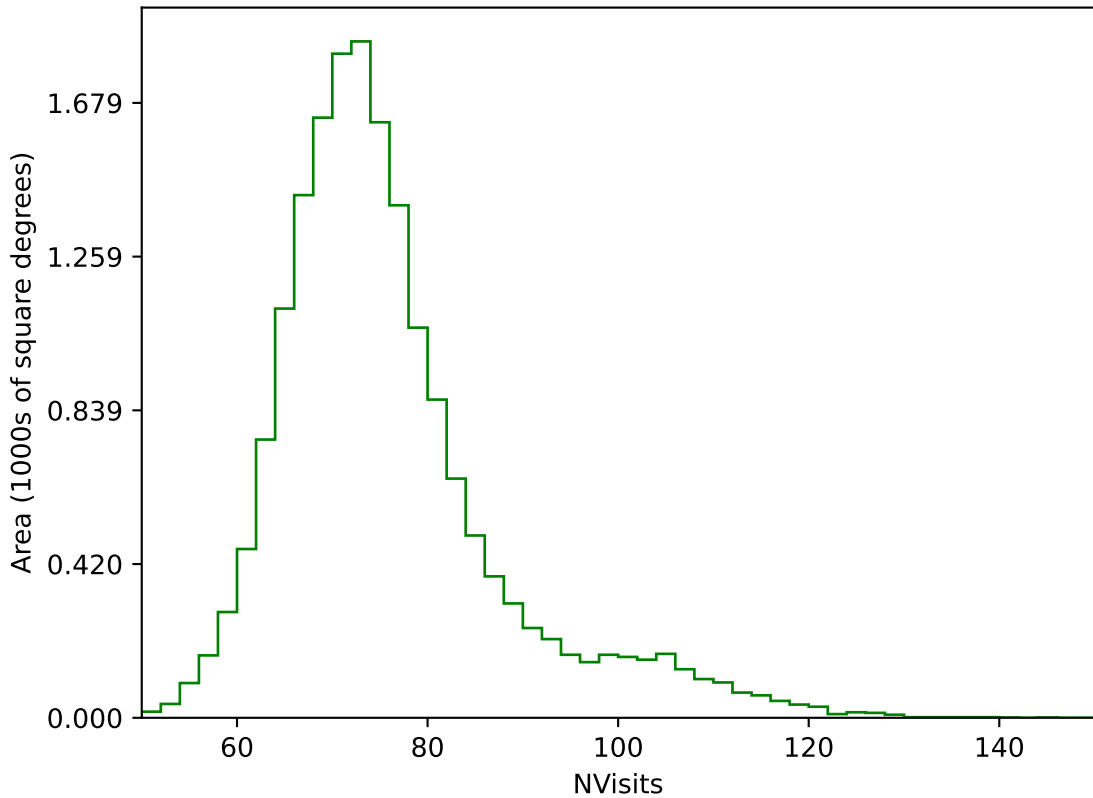
too_elab_heavy_r64_d2_gz_v3.4_10yrs WFD g band: NVisits
