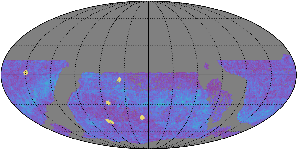
too_elab_heavy_r64_d2_gz_v3.4_10yrs WFD all bands: NVisits
