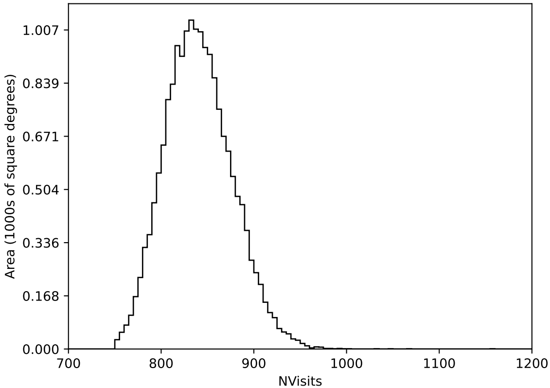
too_elab_heavy_r64_d2_gz_v3.4_10yrs WFD all bands: NVisits
