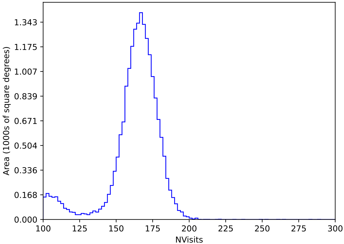
too_elab_heavy_r64_d2_gz_v3.4_10yrs All sky y band: NVisits
