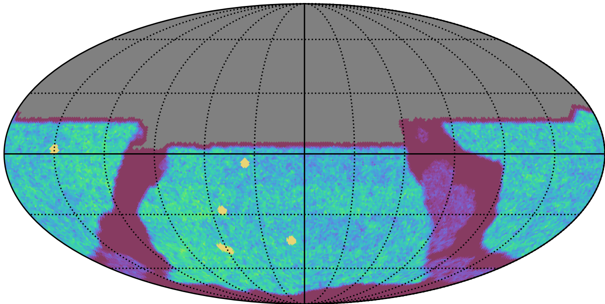
too_elab_heavy_r64_d2_gz_v3.4_10yrs All sky u band: NVisits
