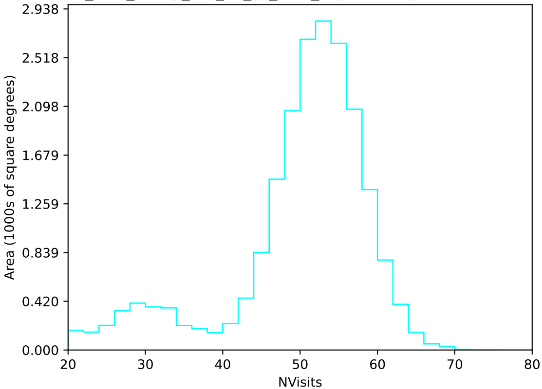
too_elab_heavy_r64_d2_gz_v3.4_10yrs All sky u band: NVisits
