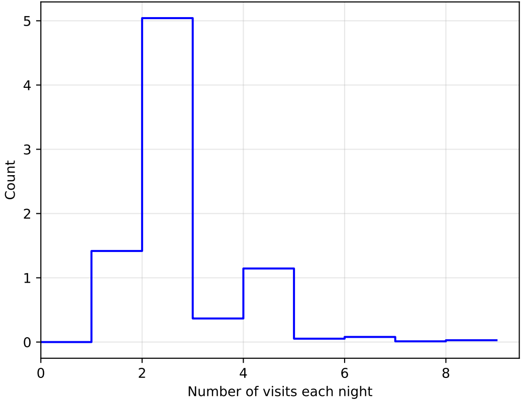
too_elab_heavy_r64_d2_gz_v3.4_10yrs WFD: NVisitsPerNight 1e6
