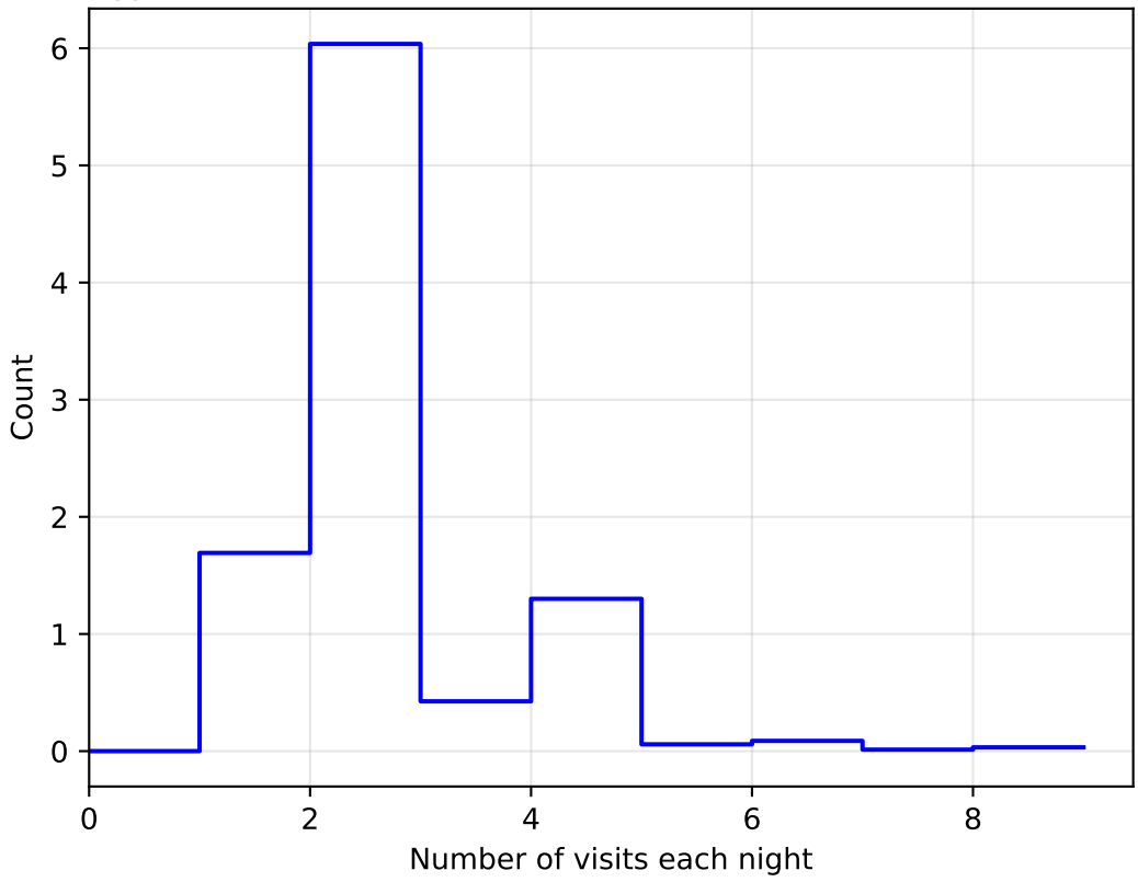
too_elab_heavy_r64_d2_gz_v3.4_10yrs All sky: NVisitsPerNight 1e6
