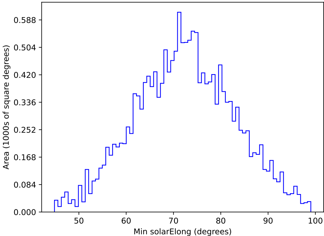
too_elab_heavy_r64_d2_gz_v3.4_10yrs WFD g band: Min solarElong
