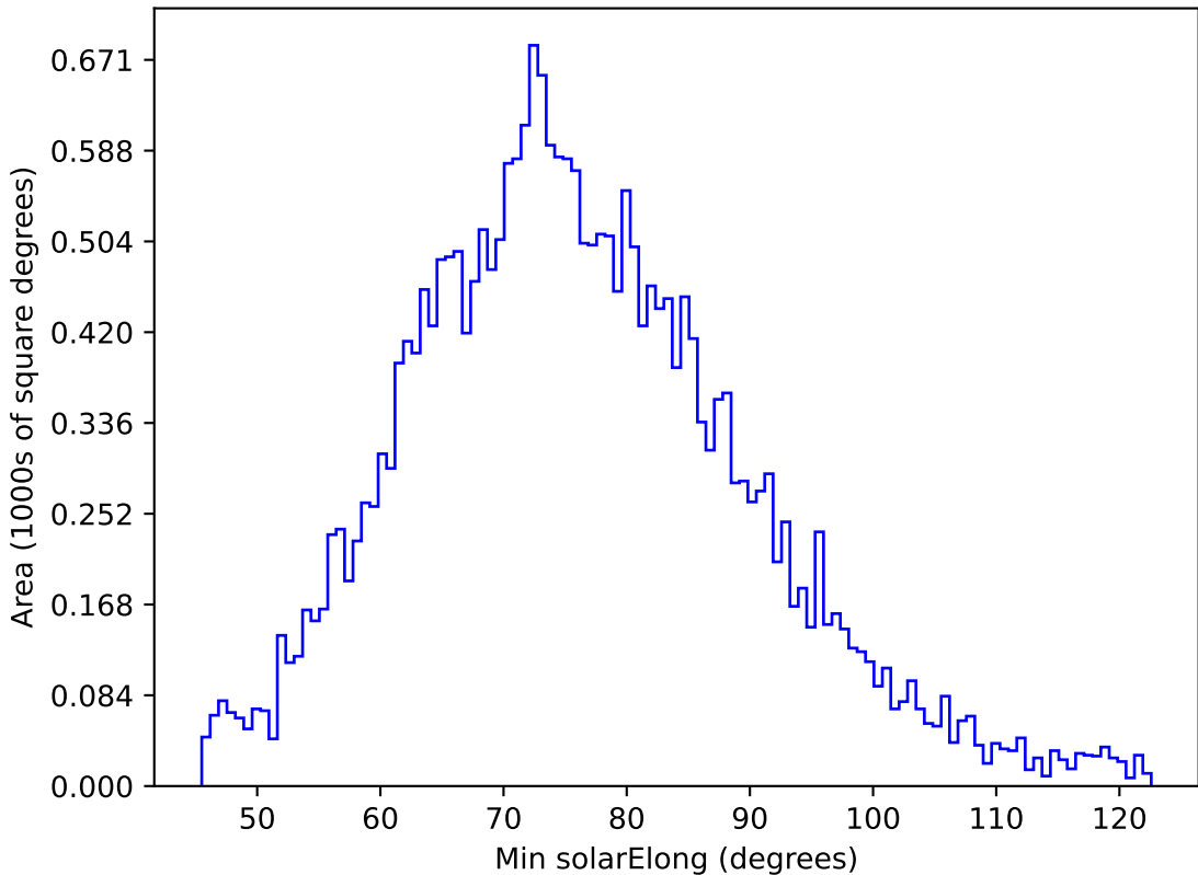
too_elab_heavy_r64_d2_gz_v3.4_10yrs All sky g band: Min solarElong
