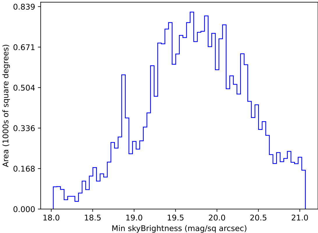
too_elab_heavy_r64_d2_gz_v3.4_10yrs Yr 1 r band: Min skyBrightness
