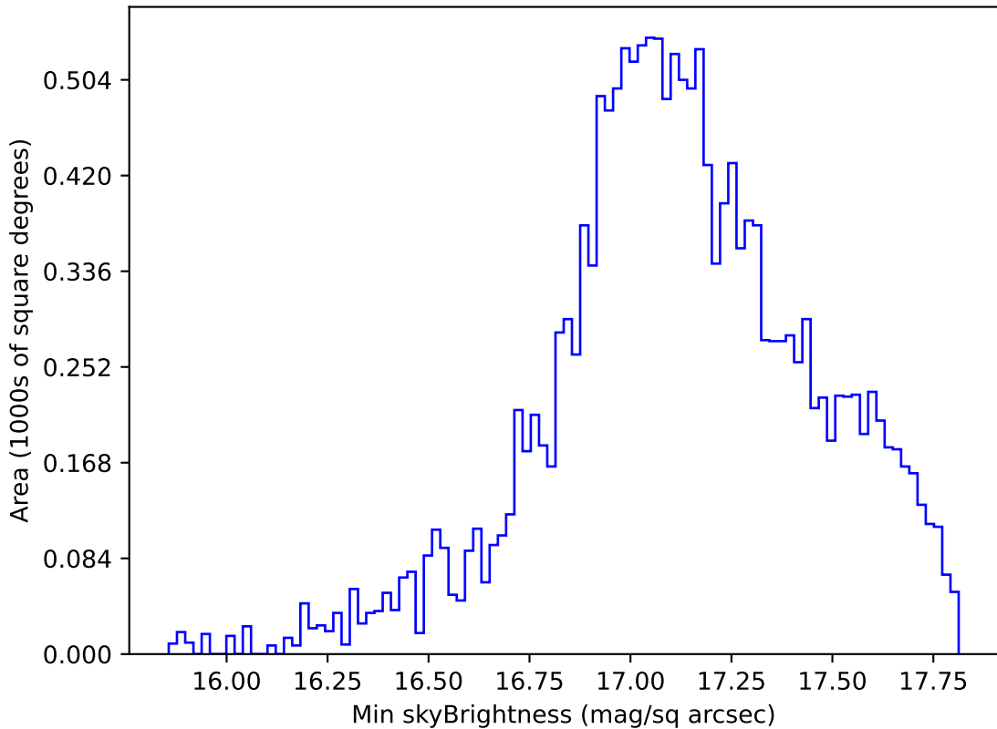
too_elab_heavy_r64_d2_gz_v3.4_10yrs WFD y band: Min skyBrightness
