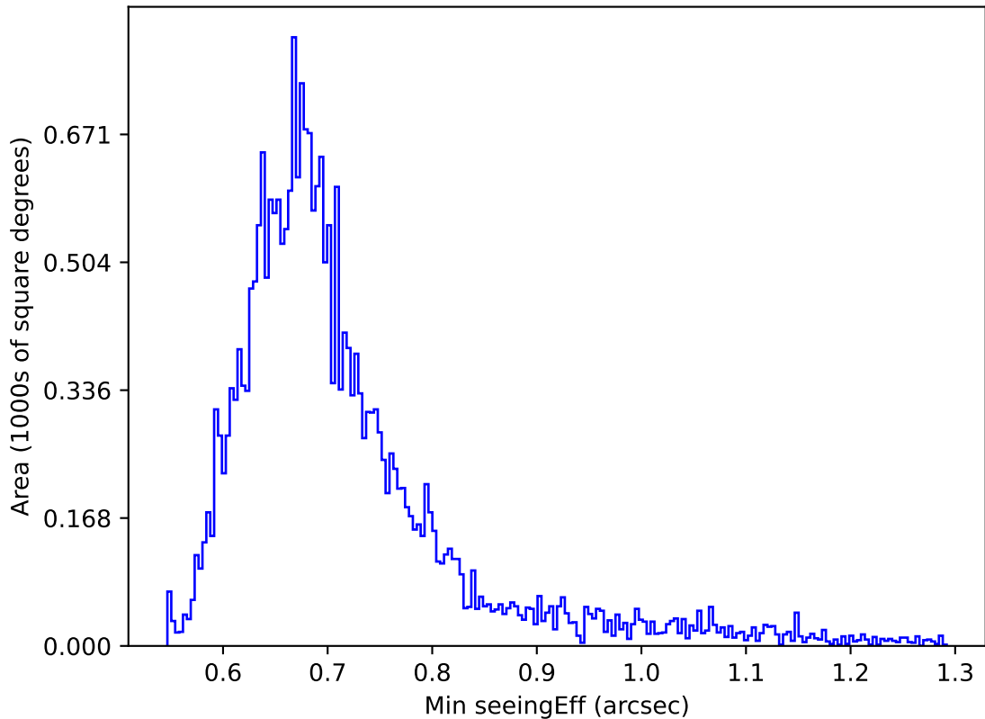
too_elab_heavy_r64_d2_gz_v3.4_10yrs Yr 1 i band: Min seeingEff
