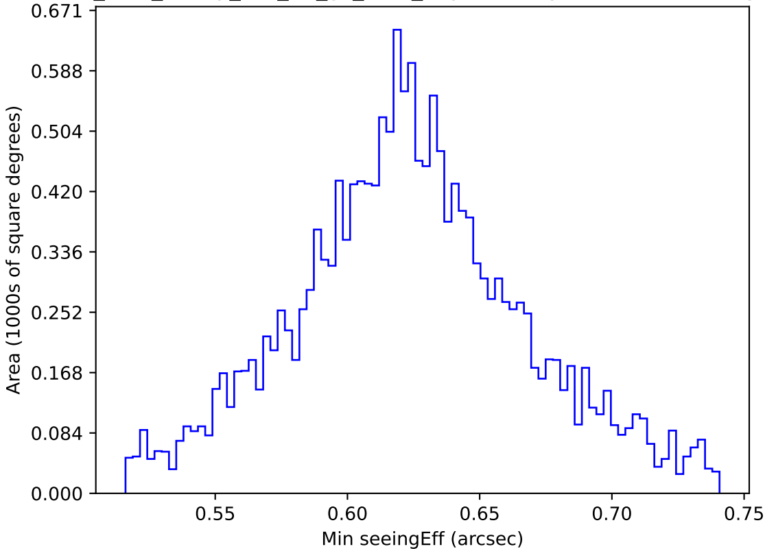
too_elab_heavy_r64_d2_gz_v3.4_10yrs WFD y band: Min seeingEff
