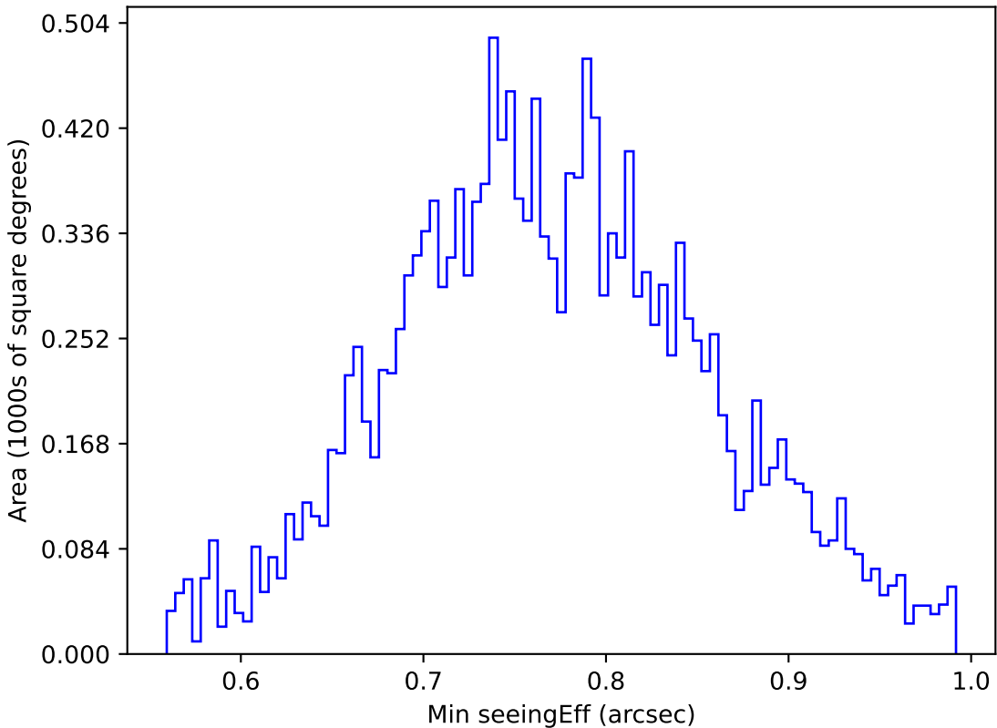
too_elab_heavy_r64_d2_gz_v3.4_10yrs WFD u band: Min seeingEff
