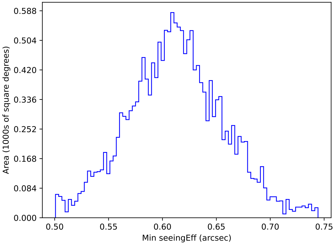
too_elab_heavy_r64_d2_gz_v3.4_10yrs WFD r band: Min seeingEff
