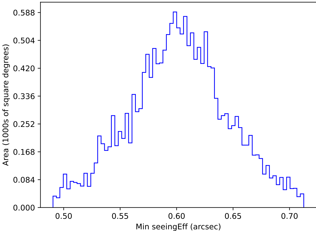
too_elab_heavy_r64_d2_gz_v3.4_10yrs WFD i band: Min seeingEff
