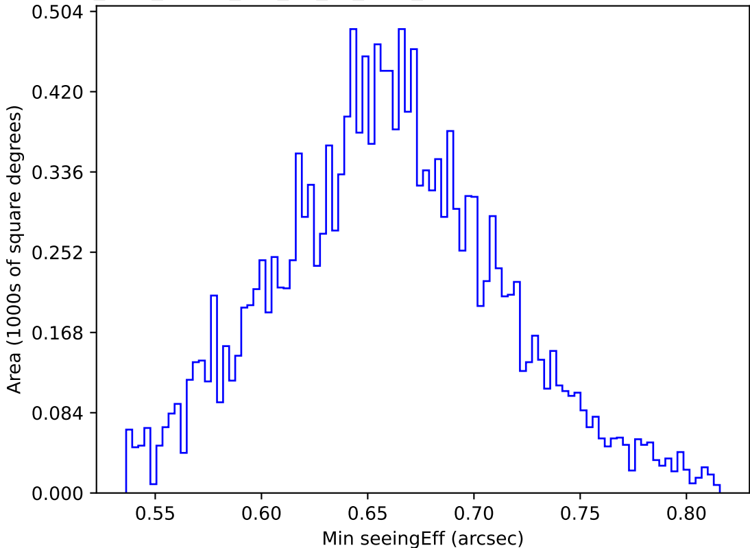
too_elab_heavy_r64_d2_gz_v3.4_10yrs WFD g band: Min seeingEff
