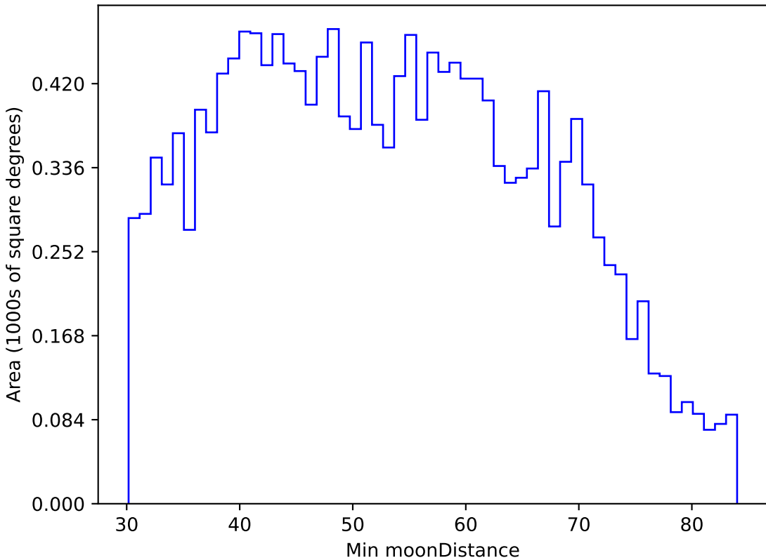
too_elab_heavy_r64_d2_gz_v3.4_10yrs WFD u band: Min moonDistance
