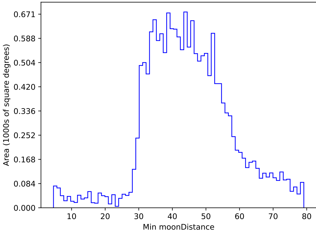
too_elab_heavy_r64_d2_gz_v3.4_10yrs WFD g band: Min moonDistance
