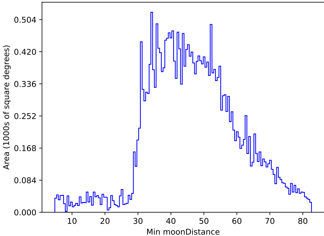
too_elab_heavy_r64_d2_gz_v3.4_10yrs All sky g band: Min moonDistance
