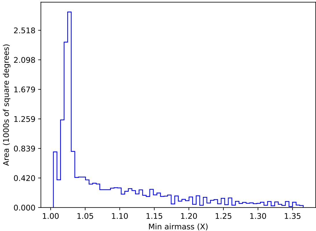
too_elab_heavy_r64_d2_gz_v3.4_10yrs WFD all bands: Min airmass
