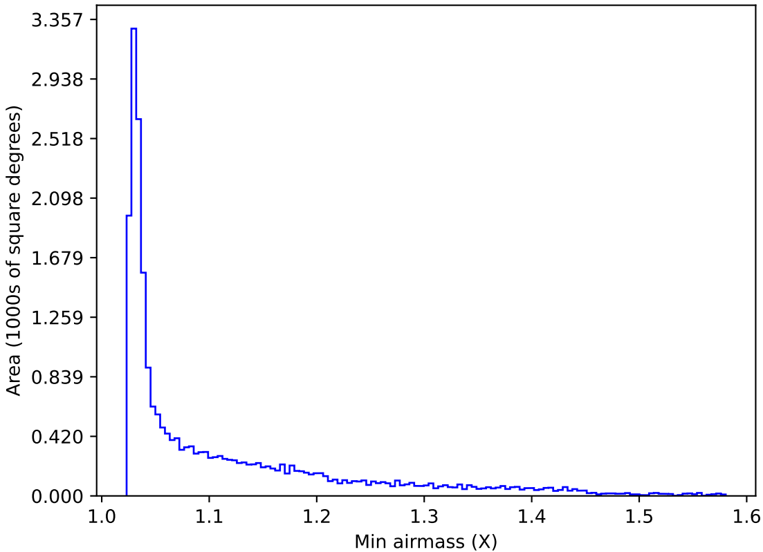
too_elab_heavy_r64_d2_gz_v3.4_10yrs All sky y band: Min airmass
