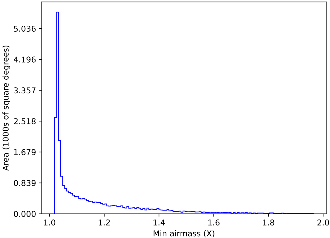
too_elab_heavy_r64_d2_gz_v3.4_10yrs All sky i band: Min airmass
