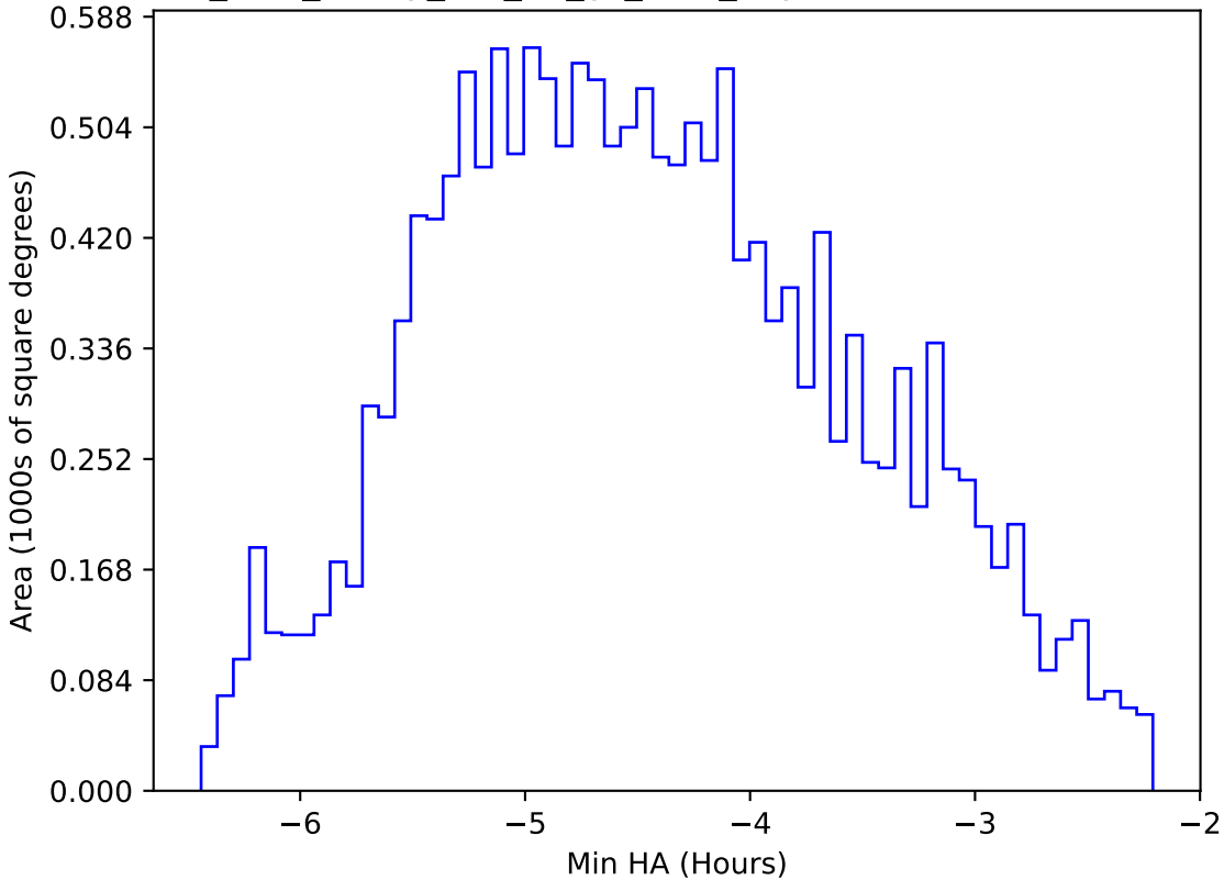
too_elab_heavy_r64_d2_gz_v3.4_10yrs WFD r band: Min HA
