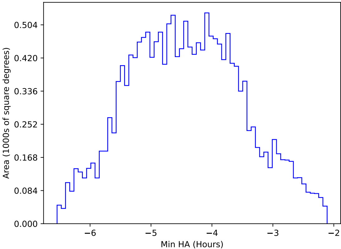
too_elab_heavy_r64_d2_gz_v3.4_10yrs WFD i band: Min HA
