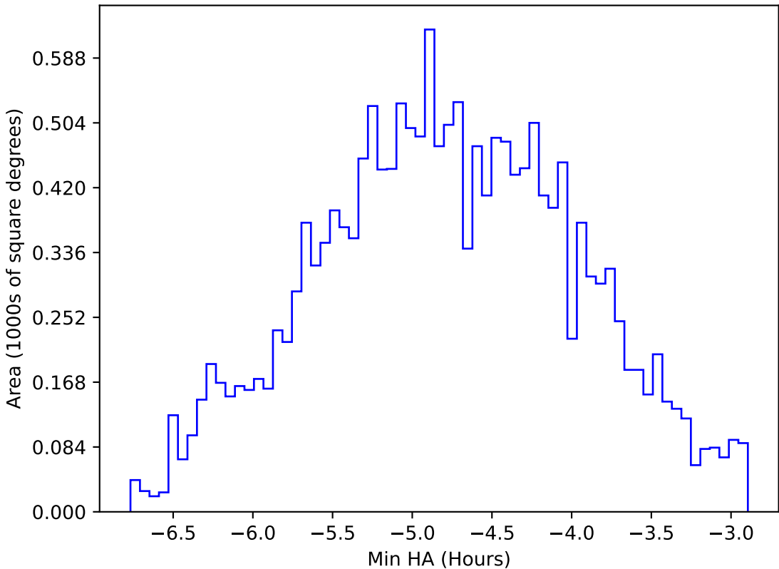
too_elab_heavy_r64_d2_gz_v3.4_10yrs WFD all bands: Min HA
