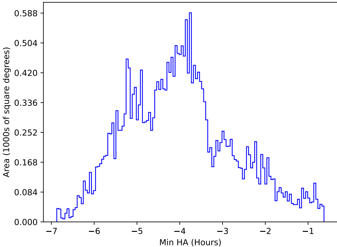
too_elab_heavy_r64_d2_gz_v3.4_10yrs All sky z band: Min HA
