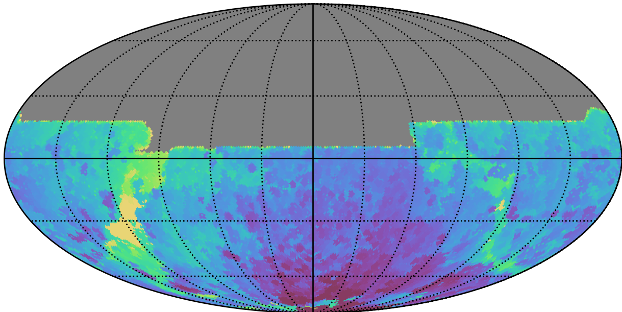
too_elab_heavy_r64_d2_gz_v3.4_10yrs All sky y band: Min HA
