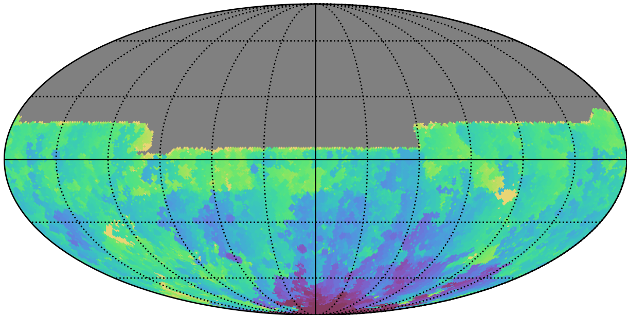
too_elab_heavy_r64_d2_gz_v3.4_10yrs All sky u band: Min HA
