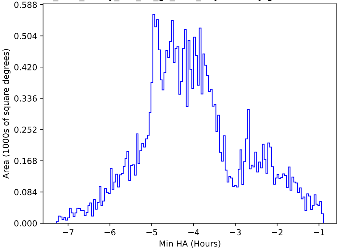
too_elab_heavy_r64_d2_gz_v3.4_10yrs All sky g band: Min HA
