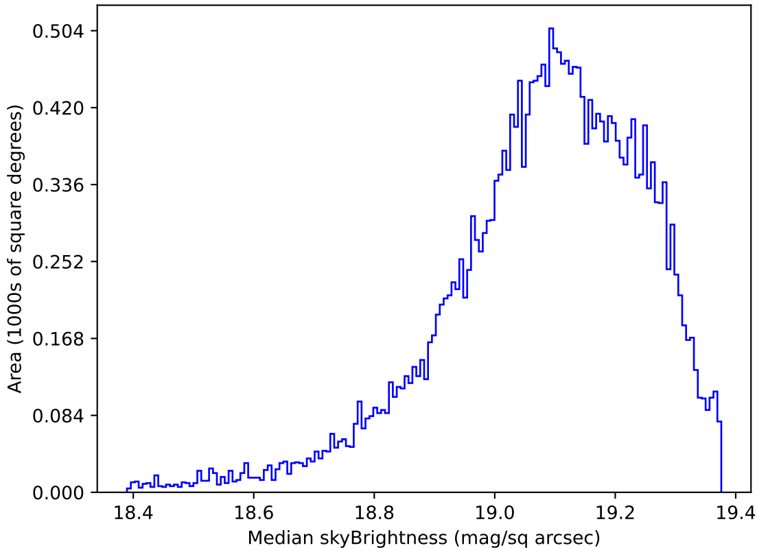
too_elab_heavy_r64_d2_gz_v3.4_10yrs Yr 1 z band: Median skyBrightness
