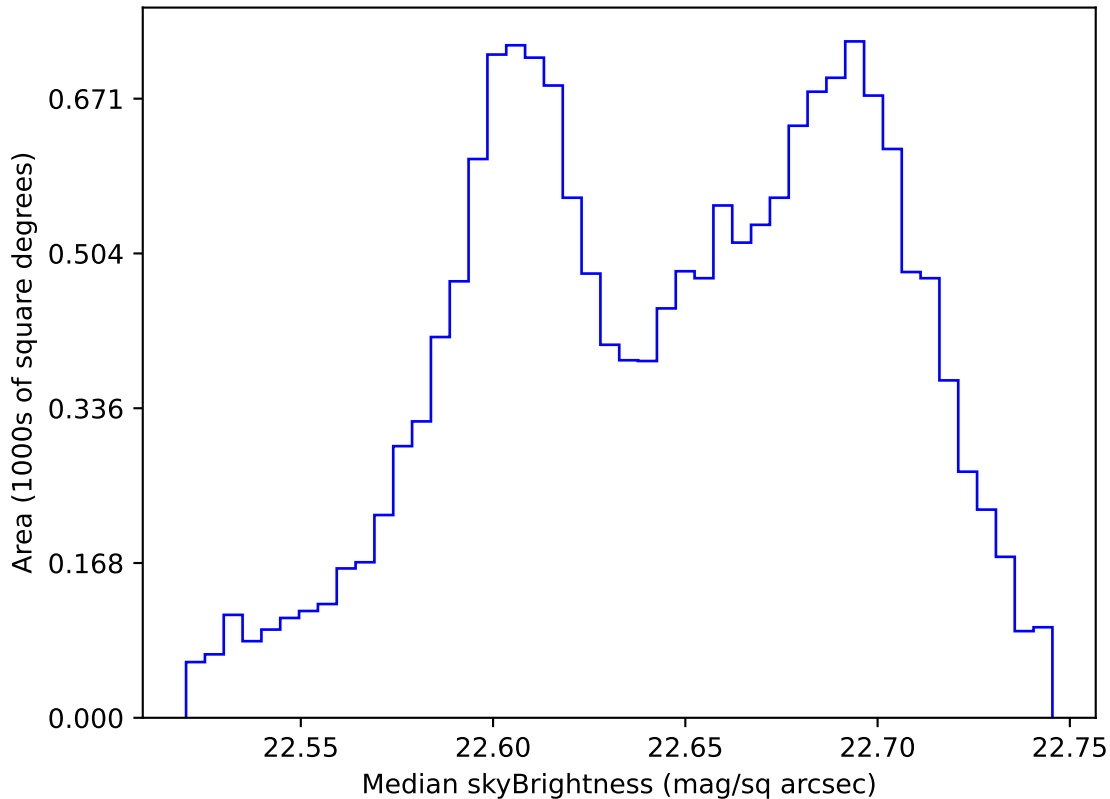
too_elab_heavy_r64_d2_gz_v3.4_10yrs WFD u band: Median skyBrightness
