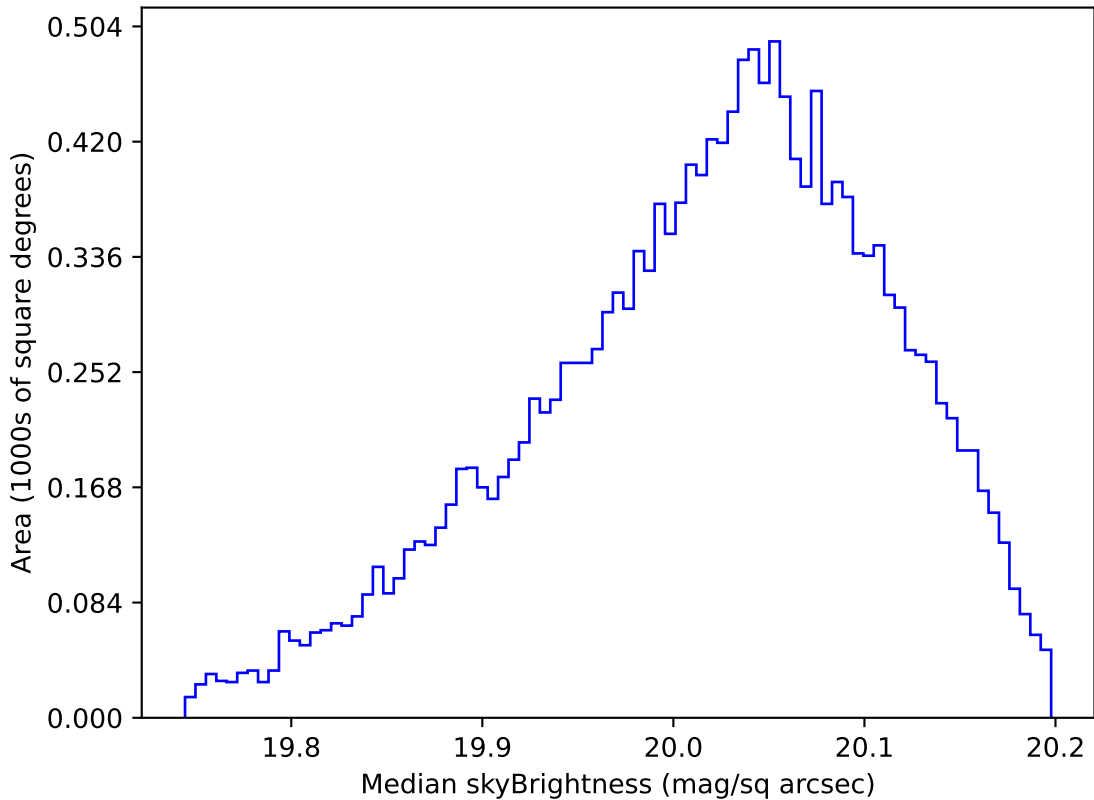
too_elab_heavy_r64_d2_gz_v3.4_10yrs WFD i band: Median skyBrightness
