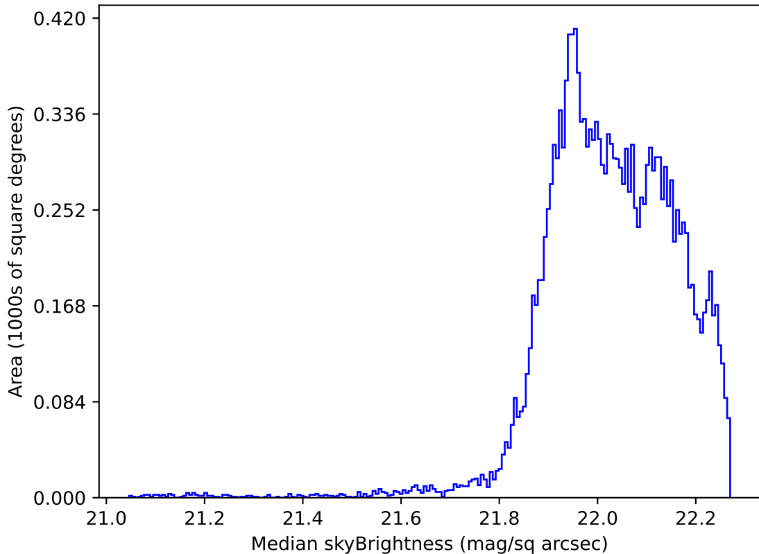
too_elab_heavy_r64_d2_gz_v3.4_10yrs WFD g band: Median skyBrightness
