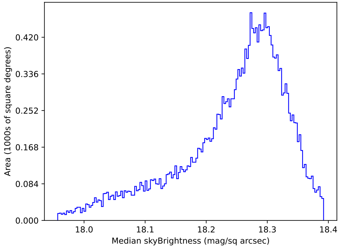
too_elab_heavy_r64_d2_gz_v3.4_10yrs All sky y band: Median skyBrightness
