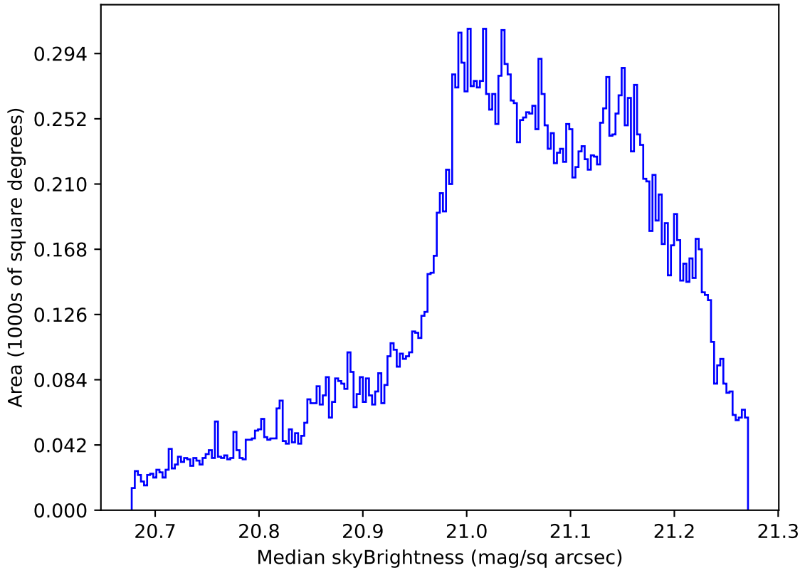
too_elab_heavy_r64_d2_gz_v3.4_10yrs All sky r band: Median skyBrightness
