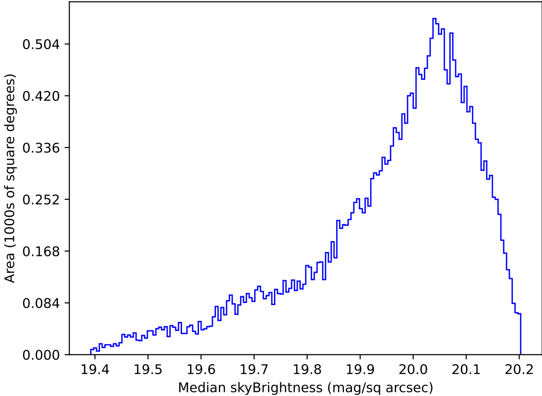
too_elab_heavy_r64_d2_gz_v3.4_10yrs All sky i band: Median skyBrightness
