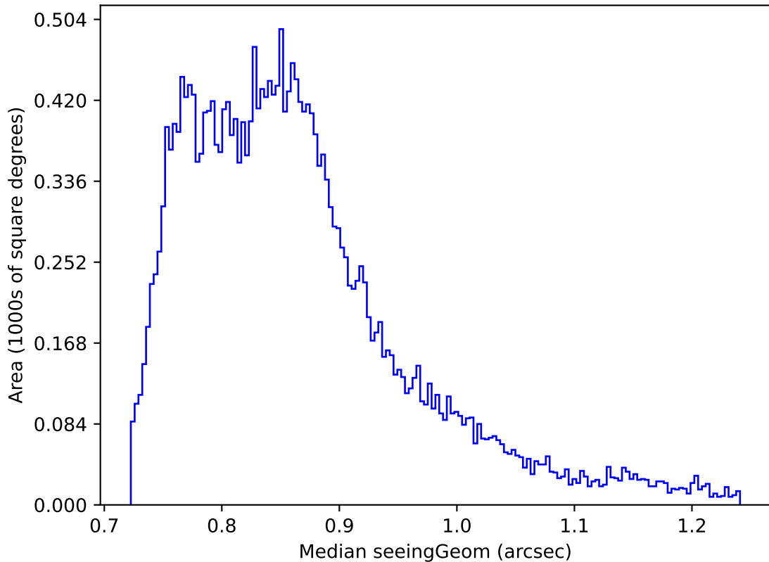
too_elab_heavy_r64_d2_gz_v3.4_10yrs Yr 1 all bands: Median seeingGeom
