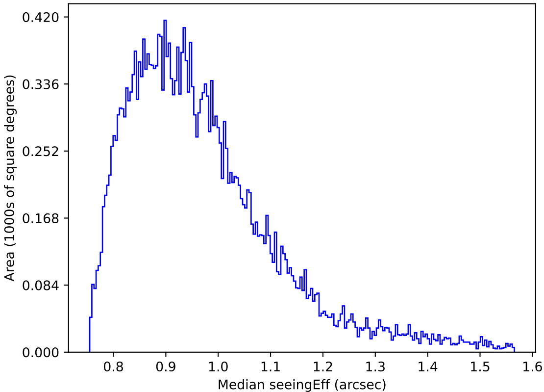
too_elab_heavy_r64_d2_gz_v3.4_10yrs Yr 1 i band: Median seeingEff
