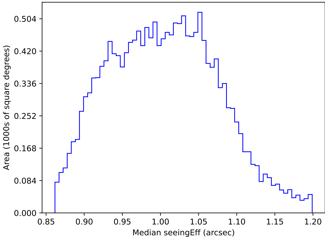
too_elab_heavy_r64_d2_gz_v3.4_10yrs WFD z band: Median seeingEff
