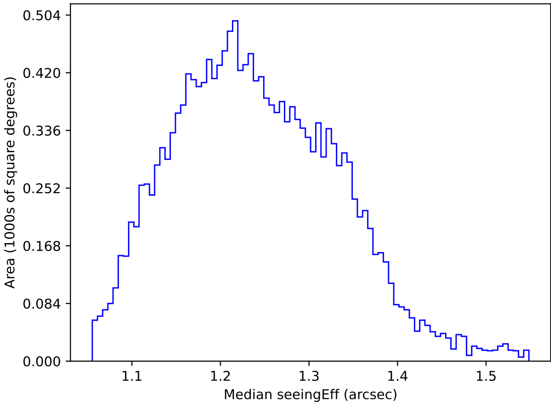
too_elab_heavy_r64_d2_gz_v3.4_10yrs WFD u band: Median seeingEff
