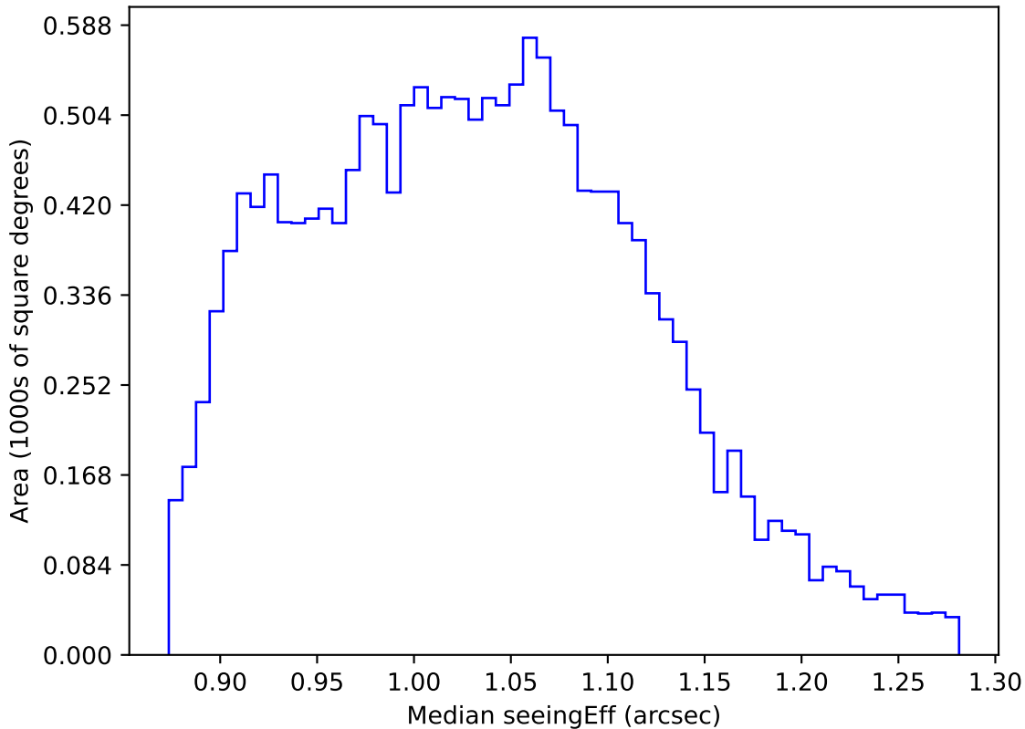
too_elab_heavy_r64_d2_gz_v3.4_10yrs WFD r band: Median seeingEff
